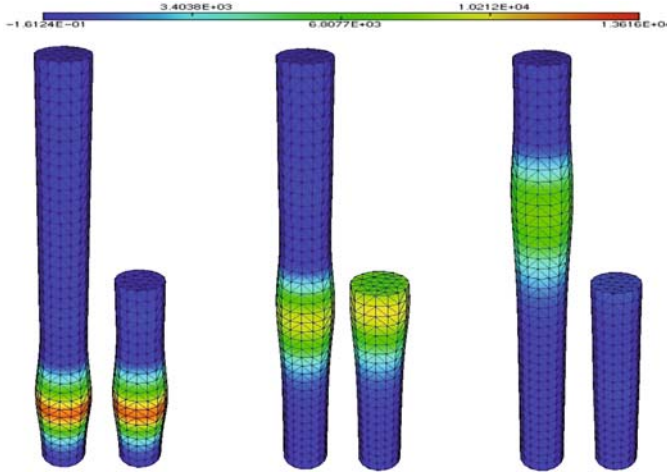
Fig. 11.27. Comparison between the pressure values of the stand-alone and the multiscale solutions at three different times ( t=0.005 , 0.01 and 0.015 ), using a 3D linear elastic model for the structure
