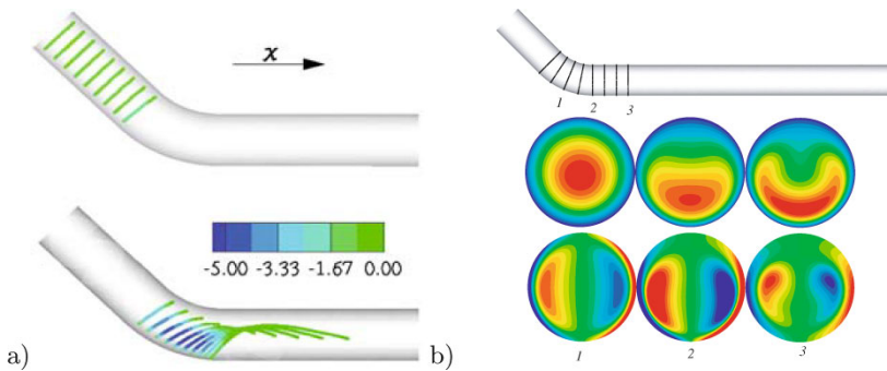
Fig. 5.8. Dean vortex generation in a single bend. (a) Ring transport and x-component vorticity stretching. (b) Sectional axial flow profile (top) and vorticity (bottom) and salient locations along the bend and exit
