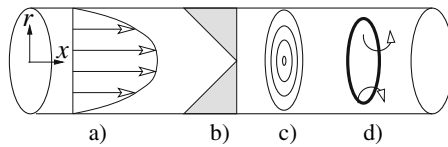
Fig. 5.6. Interpretation of Poiseuille flow in a straight pipe. a) In linear momentum terms the Poiseuille solution is a parabolic flow within the pipe, b) the parabolic velocity profile gives rise to a linear variation of vorticity across the pipe, c) an alternative local rotational momentum (vorticity) interpretation of the flow is a series of ring of varying circulation, d) from a modelling point of view we can consider an isolated ring with a lumped vorticity
