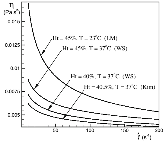
Fig. 6.7. Comparison of viscosity functions \mu(\dot{\gamma}) for the power-law model (6.21) using material constants provided by Kim et al. [258] (Kim) and Liepsch and Moravec [288] (LM) for human blood. Also shown are representative viscosity curves for the Walburn-Schneck model (WS) [534] that includes a dependence on haematocrit (6.22). Values for the material constants n and k are given in Table 6.1
