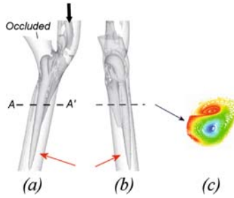
Fig. 5.21. Left: Vortical flow structures at distal anastomosis of aorto-coronary graft. Although the global geometry is that of a shallow S-bend, localised constriction produces highly asymmetric flow shown by dominant vortex core. Right: Distribution of particles (coded by distance from centreline radius at inflow) at indicated section AA'
