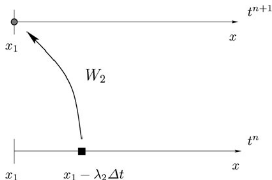
Fig. 10.2. Extrapolation of the characteristic W_2 in x_1
