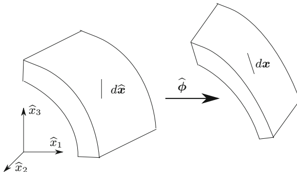
Fig. 3.1. Local deformation of a material neighbourhood. An infinitesimal vector d\hat{x} is deformed into dx
