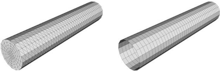
Fig. 12.11. The fluid and solid computational meshes: 21534 tetrahedra for the fluid and 640 quadrilaterals for the solid
