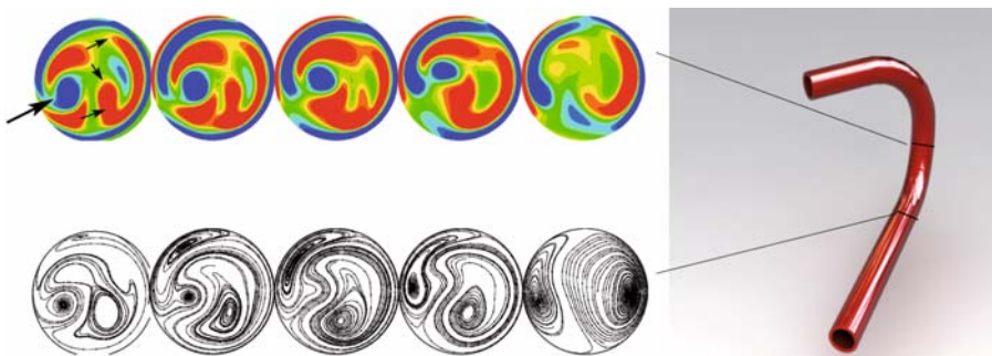
Fig. 5.13. Vortex merging and cancellation in non-planar 135^\circ sequence of bends at Re_D=500
