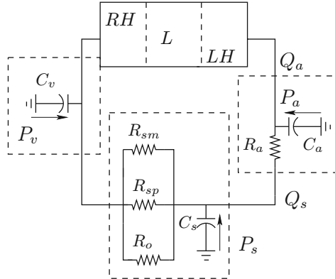
Fig. 10.17. Simplified compartment model of the circulation
