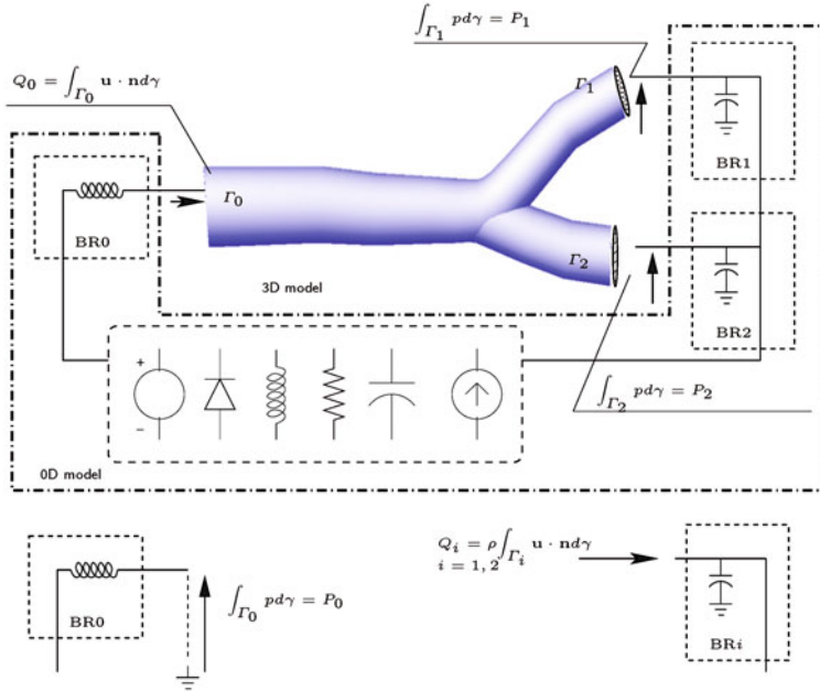
Fig. 11.12. Representation of a 3D rigid-0D geometrical multiscale model with three bridging regions (BR0, BR1, BR2). At the inlet of the 3D domain, the bridging region has the current/flow rate Q_0 as state variable. The latter is computed by the 0D model and provided to the NS model. In the other bridging regions, the voltage/pressures p_i , i = 1, 2 , are the state variables. The 0D model is forced by the mean pressure at the interface \Gamma_0 and by the flow rates at \Gamma_1 and \Gamma_2
