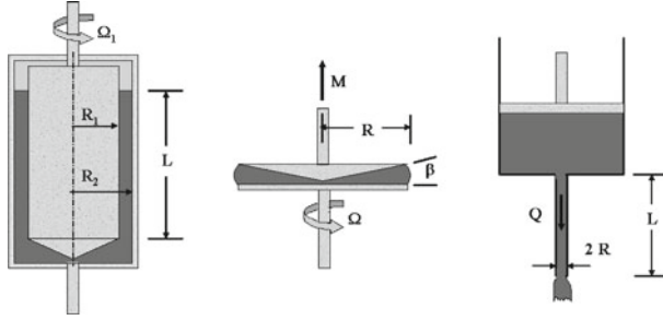
Fig. 6.4. Schematic of three rheometers commonly used for blood: (a) Couette, (b) cone and plate, and (c) capillary
