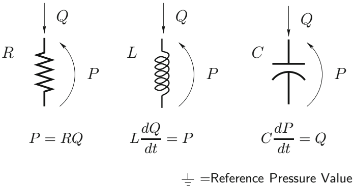
Fig. 10.6. Notation used in the electrical analogy of the circulatory system
