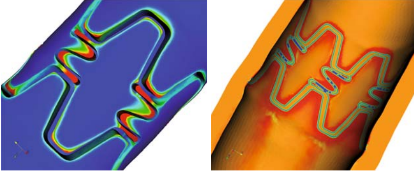
Fig. 12.16. The contour plots of the concentration on the surface of the arterial lumen at 40 seconds after the beginning of the process are shown on the left. The colour scale ranges linearly from 0 (blue) to 10^{-3}c_s^0 (red). The mass flux exchanged between the lumen and the arterial wall is shown on the right. The red colour denotes a positive flux from the lumen to the wall, while the blue colour refers to the opposite case
